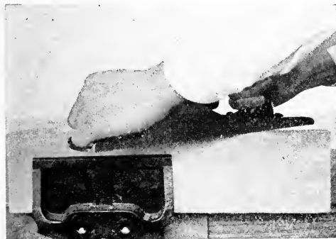
Fig. 39—Swinging Plane on Return Stroke
